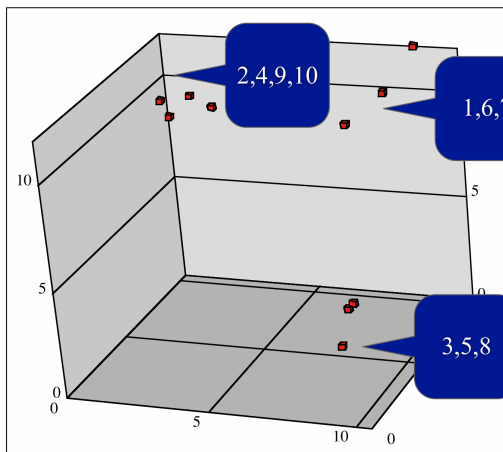
PAIRWISE DISTANCES
